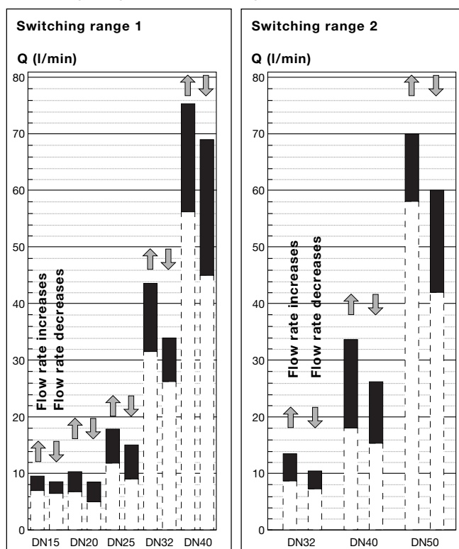
Switching range table for fitting PVC, PVDF, PP, SS, Brass
