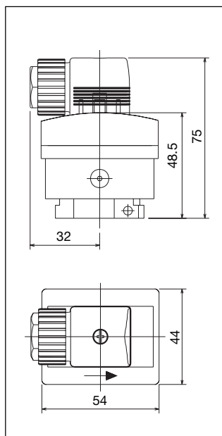
Dimensions [mm]
