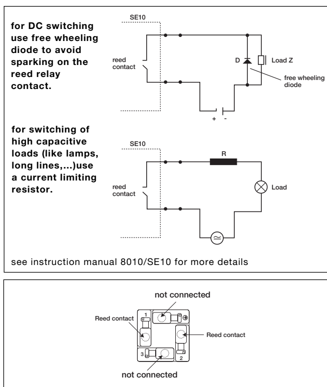
Electrical connection - Reed contact version
